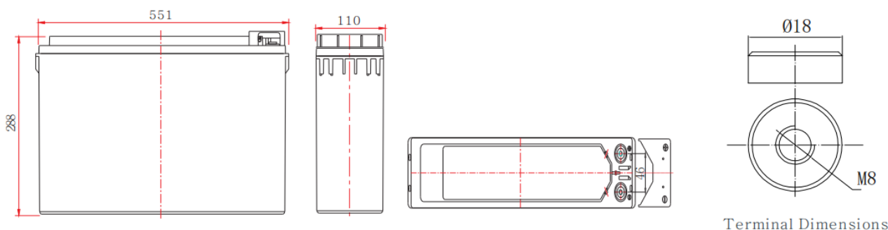
Terminal Dimensions
