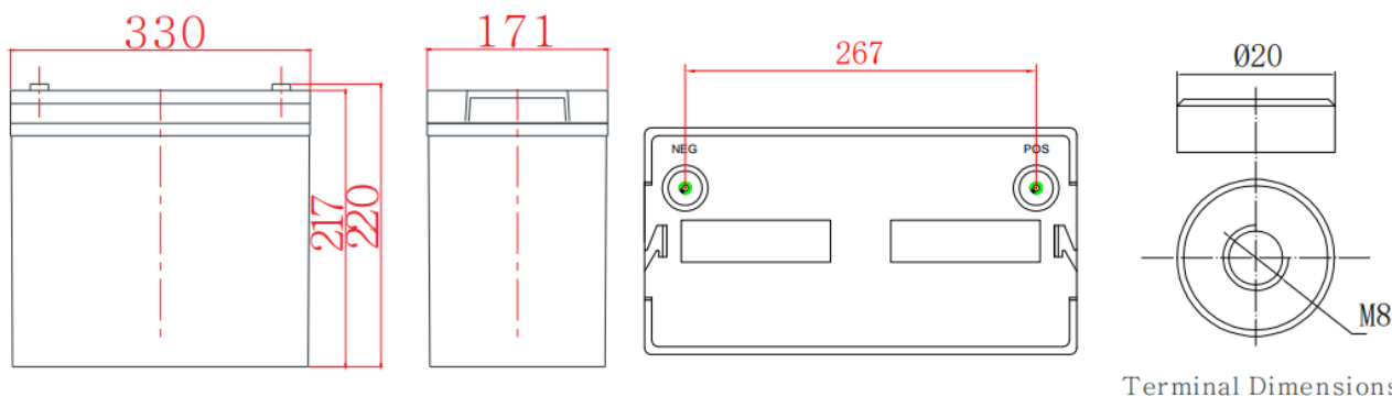
Terminal Dimensions
