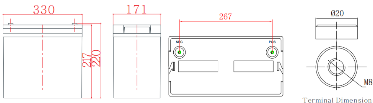
Terminal Dimensions
