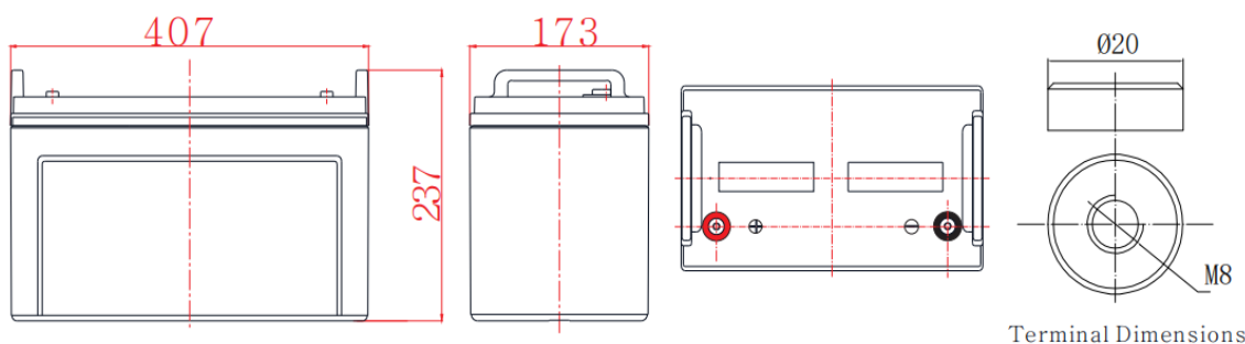
Terminal Dimensions
