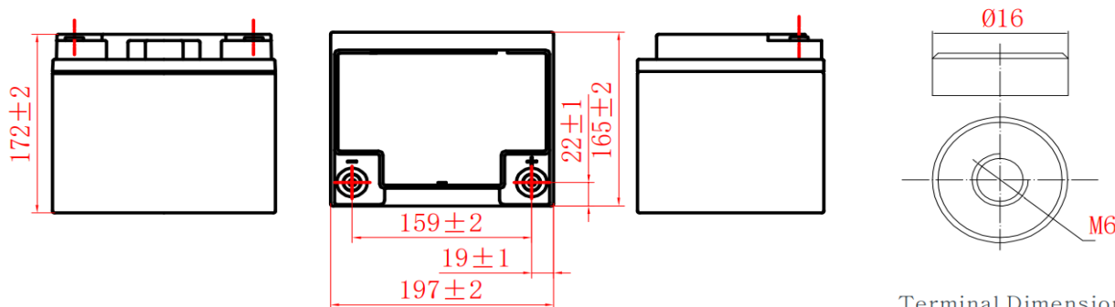
Terminal Dimensions
