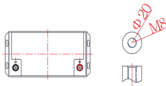
Terminal Dimensions
