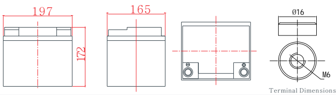
Terminal Dimensions
